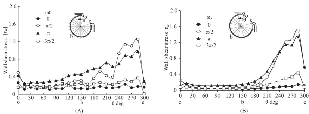
Fig. 7. Normalized and absolute wall shear stress along aneurysm wall of elastic model in pulsatile flow. Re_m = 435 , \alpha = 4.0 , A = 0.68 . (A) PIV; (B) CFD.
