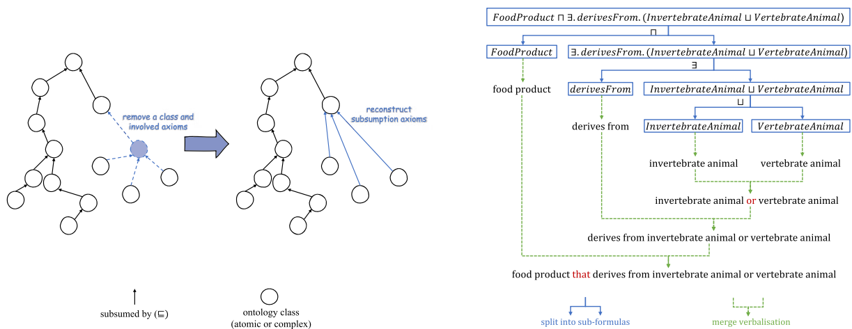
Fig. 2. The left figure illustrates the process of removing a concept while preserving the subsumption hierarchy in the ontology pruning algorithm proposed in Bio-ML [19]. The right figure illustrates an example of the application of the recursive concept verbalisation algorithm proposed in OntoLAMA [20].
