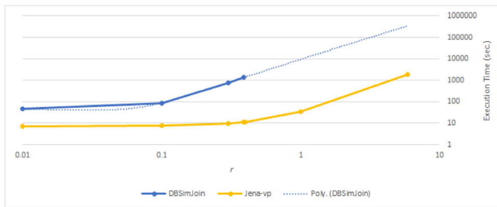
Fig. 17. Execution time of range-based self-similarity joins, including polynomial trend line for DBSimJoin times beyond r = 0.4 .
