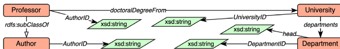
Fig. 1. Example of an ontology of the university domain including 4 concepts and relationships among them, as well as relationships between concepts and datatypes.
