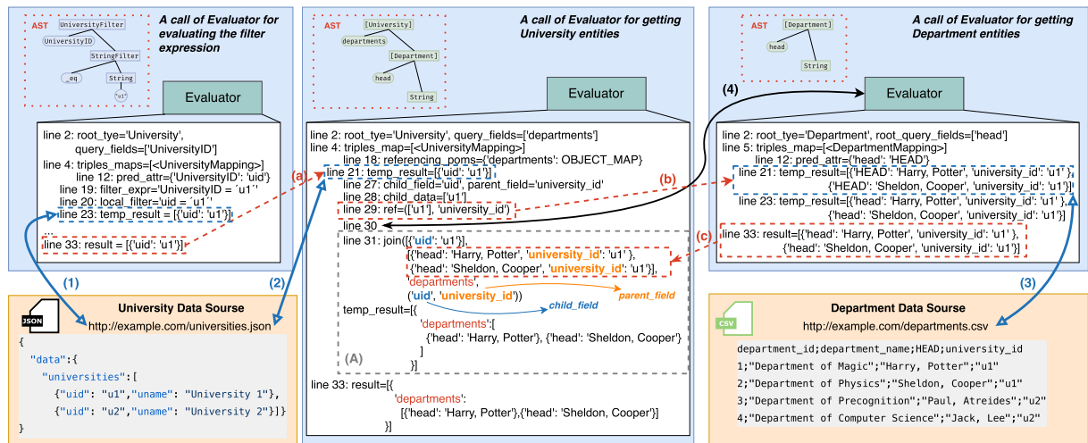
Fig. 5. Example for answering the query in Listing 3. (1) – (3) indicate the requests to and responses from the data sources; (a) – (c) indicate the parameter passing between the calls to evaluators ; (4) indicates a recursive call to evaluator for getting the data of departments ; frame (A) indicates a join operation.
