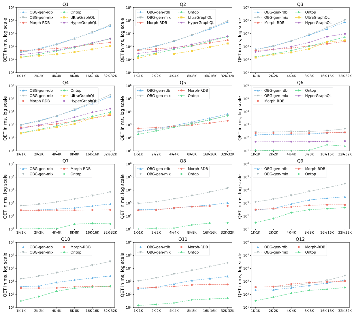
Fig. 8. Query Execution Time (QET) per query on materials dataset.
