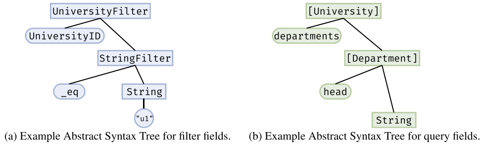
Fig. 3. Example abstract syntax trees for the query shown in Listing 3.
