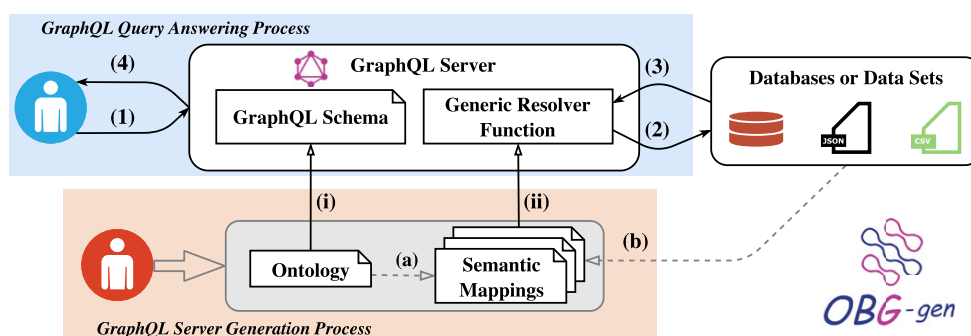
Fig. 2. GraphQL-based framework for data access and integration.
