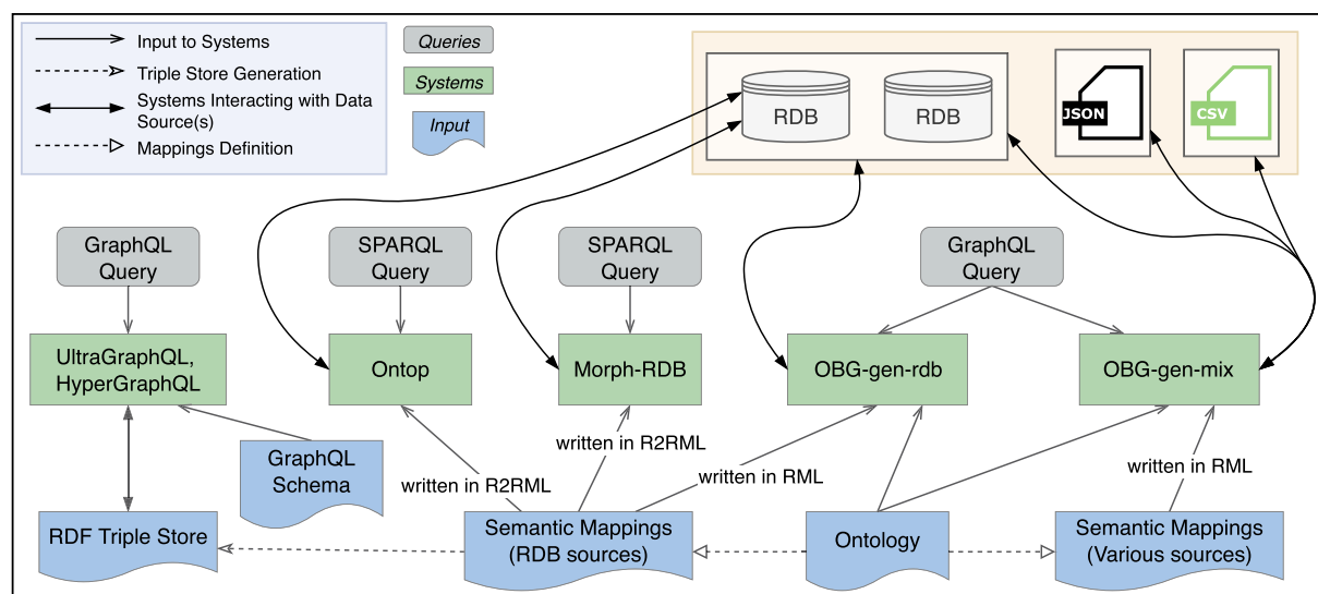
Fig. 7. Outline of the real case evaluation.
