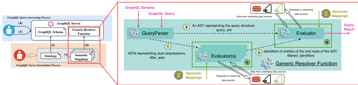
Fig. 4. Technical components in the generic resolver function.
