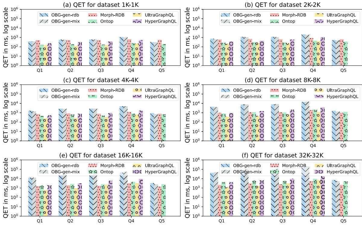
Fig. 9. Query Execution Time (QET) per data size on materials dataset for queries without filtering conditions.
