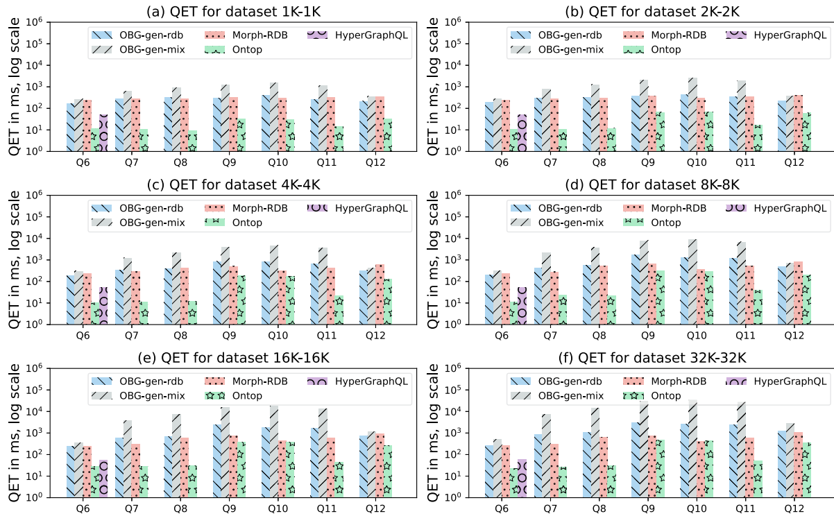
Fig. 10. Query Execution Time (QET) per data size on materials dataset for queries with filtering conditions.
