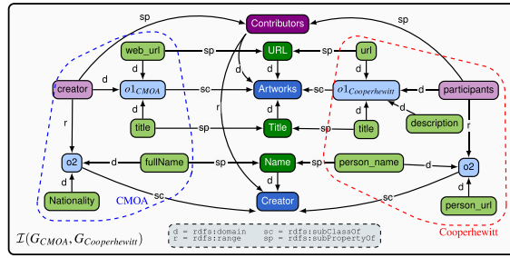
Fig. 13. Final integration graph from Examples 4 and 5.
