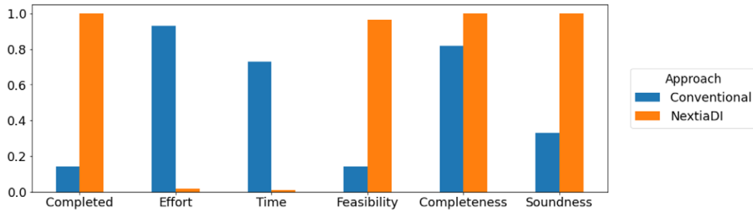
Fig. 24. Aggregated results for the mapping generation phase. Completed specifies whether participants finished the task within the available time (higher is better). Effort and Time indicate, respectively, the perceived effort and time to complete the task (lower is better). Feasible is used to quantify the perceived feasibility of the task in Big Data settings (higher is better). Completeness and Soundness refer to the quality metrics previously introduced.
