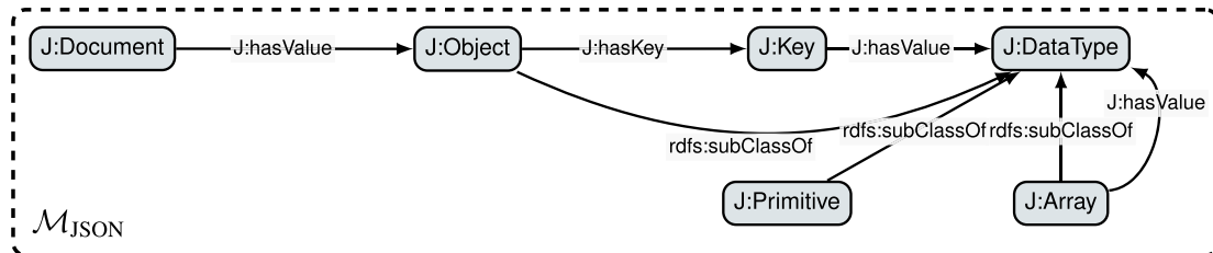
Fig. 5. Metamodel to represent graph-based schemata of JSON datasets (i.e., \mathcal{M}_{\text{JSON}} ) inspired from [29].
