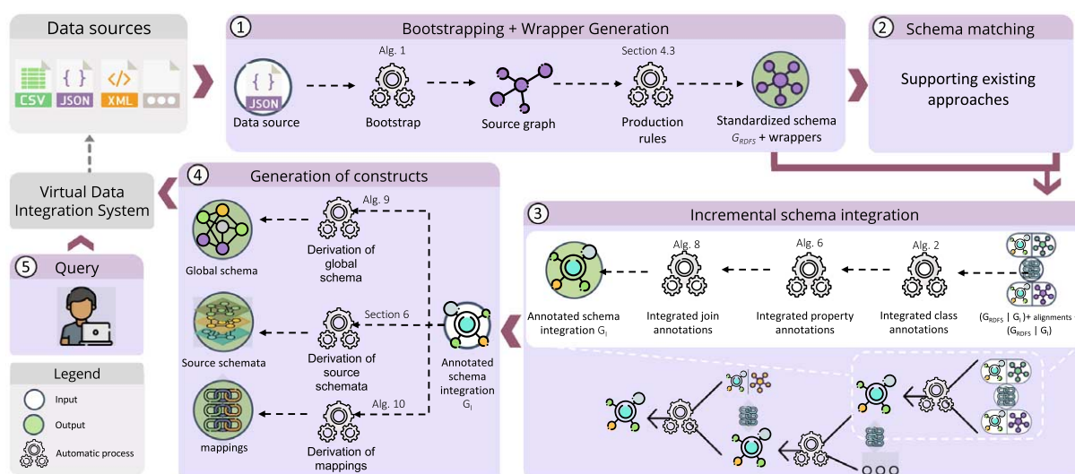
Fig. 2. Our approach in a nutshell.
