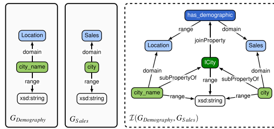
Fig. 14. Example of a join integration.
