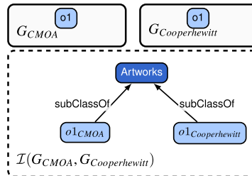
Fig. 11. Integration of two classes from G_{CMOA} and G_{Cooperhewitt} .
