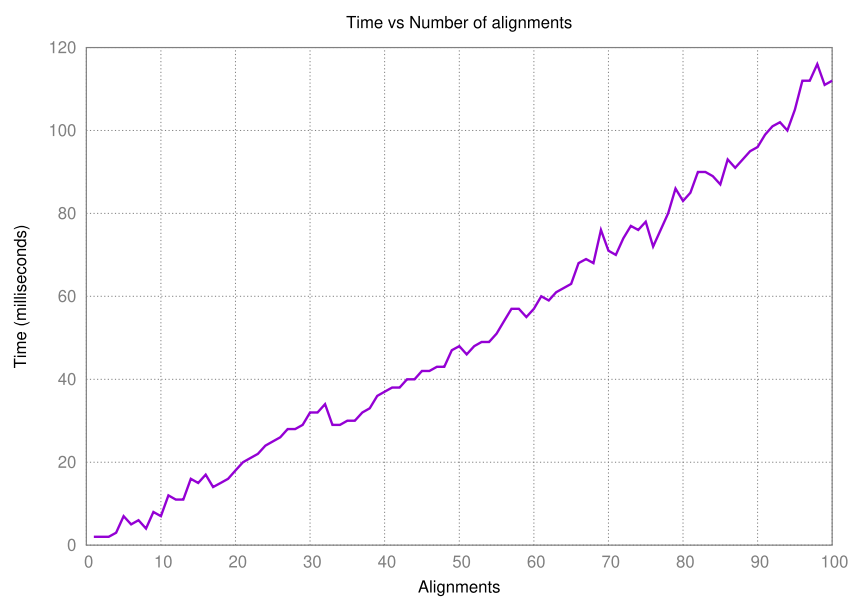
Fig. 26. Performance evaluation when alignments increased incrementally.
