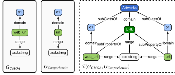
Fig. 12. Result of integrating two classes and two data type properties from G_{CMOA} and G_{CooperhewittInt} .
