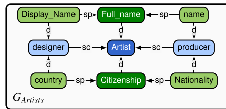
Fig. 15. New data source.
