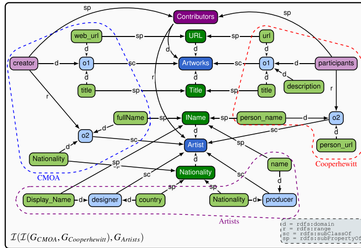
Fig. 18. Integration graph from a second integration.
