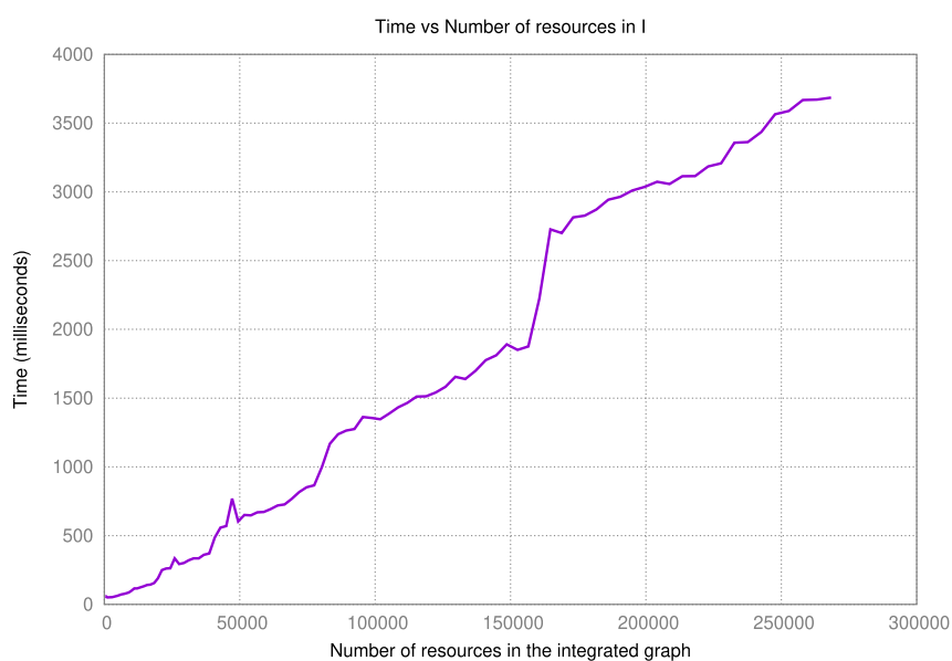
Fig. 27. Performance evaluation when the number of schema elements increased.
