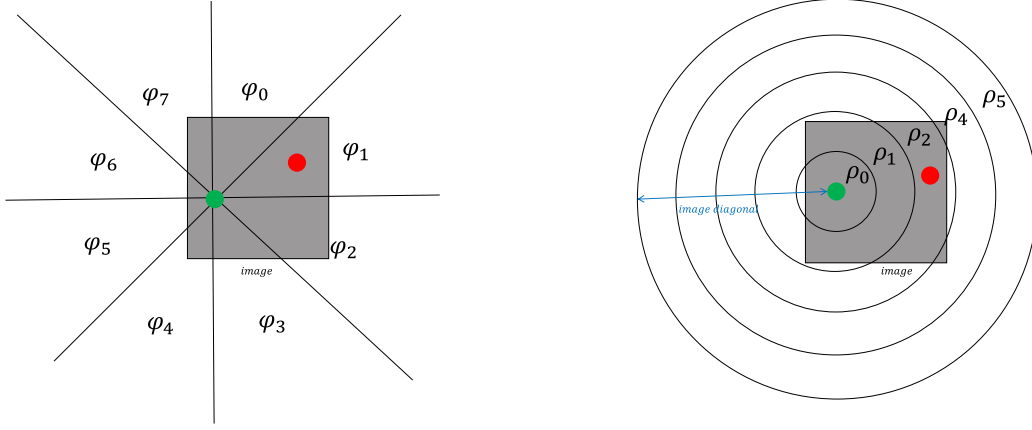
Fig. 12. Spatial neural predicates explanation by examples. Left: directions of red circle with respect to green circle denoted by symbols \phi_1, \dots, \phi_7 . The red circle is in the direction of \phi_1 . Right: distance of red circle to the green circle denoted by the symbols \rho_1, \dots, \rho_5 . The red circle is located at the distance of \rho_2 . For 3D KP, we assume all the object placed on a flat surface with same height. Thus their positions can be mapped to 2D space with ignoring the axis denoting the height. The positions of each object can be evaluated from depth map of 3D scenes.
