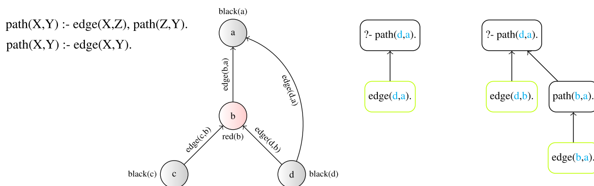
Fig. 2. An example learned ILP model of a path (left), being unfolded on a labeled graph sample encoded in relational logic (middle), resulting into two different computation graphs for the same target query “path(d, a)” (right).
