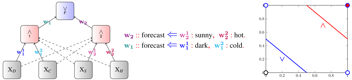
Fig. 1. An example correspondence between a neural network (left) and a propositional logic program (middle), based on conjunctive and disjunctive activations emulated by the respectively weighted neurons (right), in the spirit of KBANN [50].
