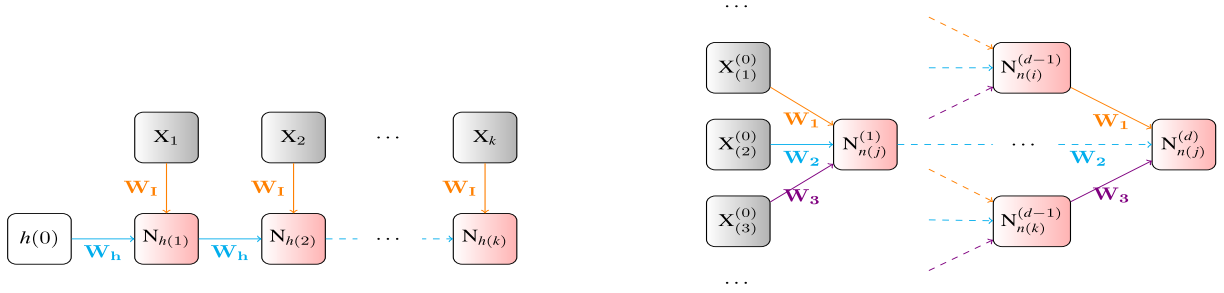
Fig. 4. The symmetric weight-sharing patterns in the structured computation graphs of recurrent (left) and recursive (right) neural models.
