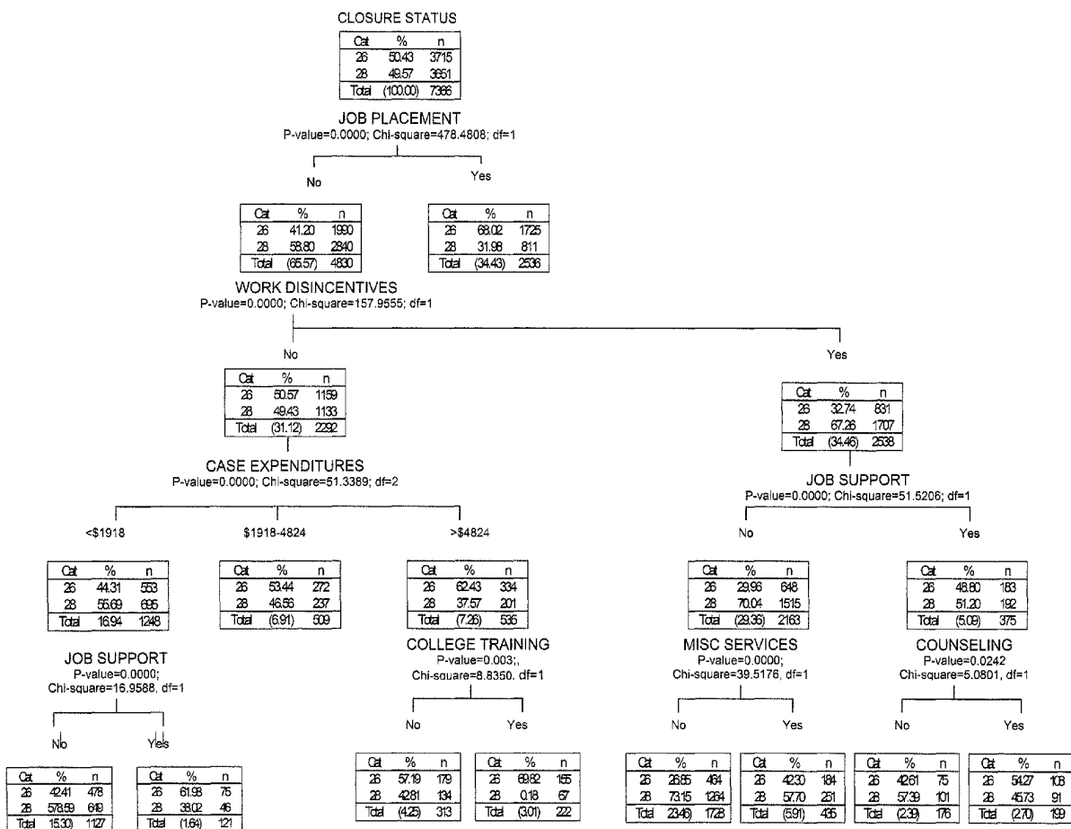
Fig. 2. CHAID diagram of the partial tree depicting factors predicting subgroups of individuals who did not receive job placement assistance.
