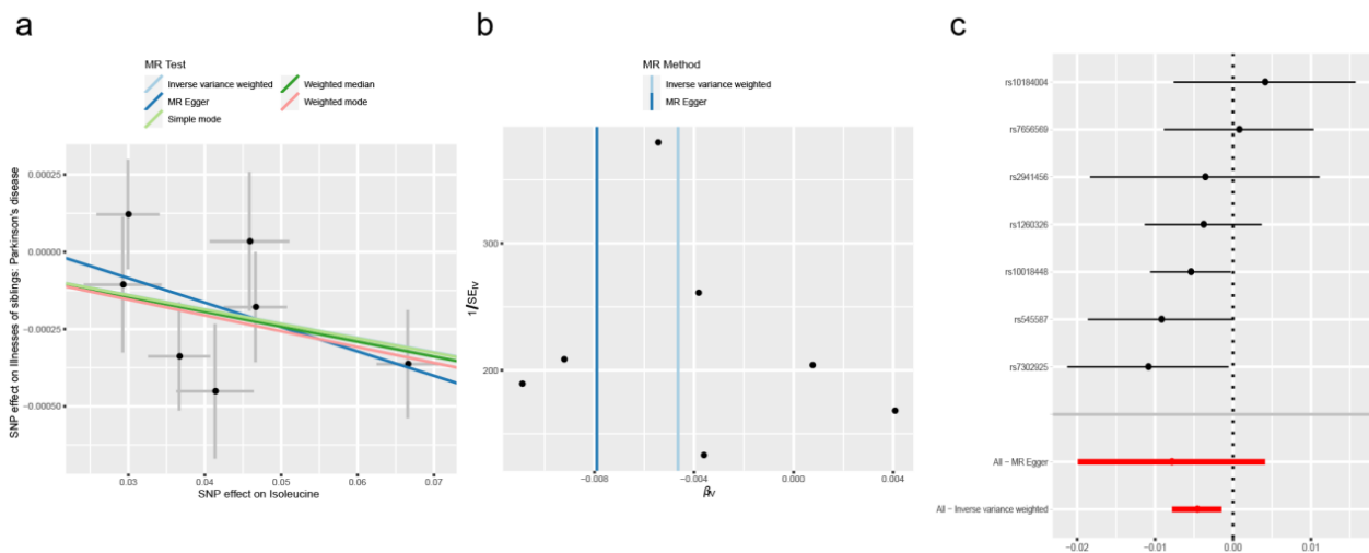
Supplementary Figure 2. The causal effect of isoleucine on PD risk. (a) Scatter plot, (b) Funnel plot and (c) Forest plot. PD, Parkinson's disease.
