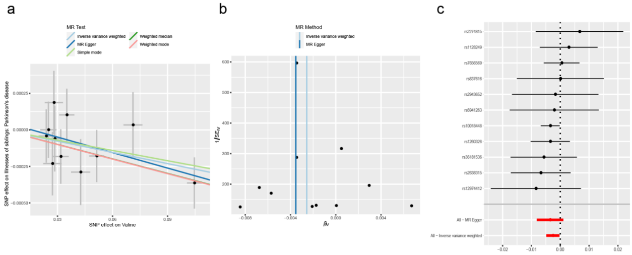
Supplementary Figure 3. The causal effect of valine on PD risk. (a) Scatter plot, (b) Funnel plot and (c) Forest plot. PD, Parkinson's disease.
