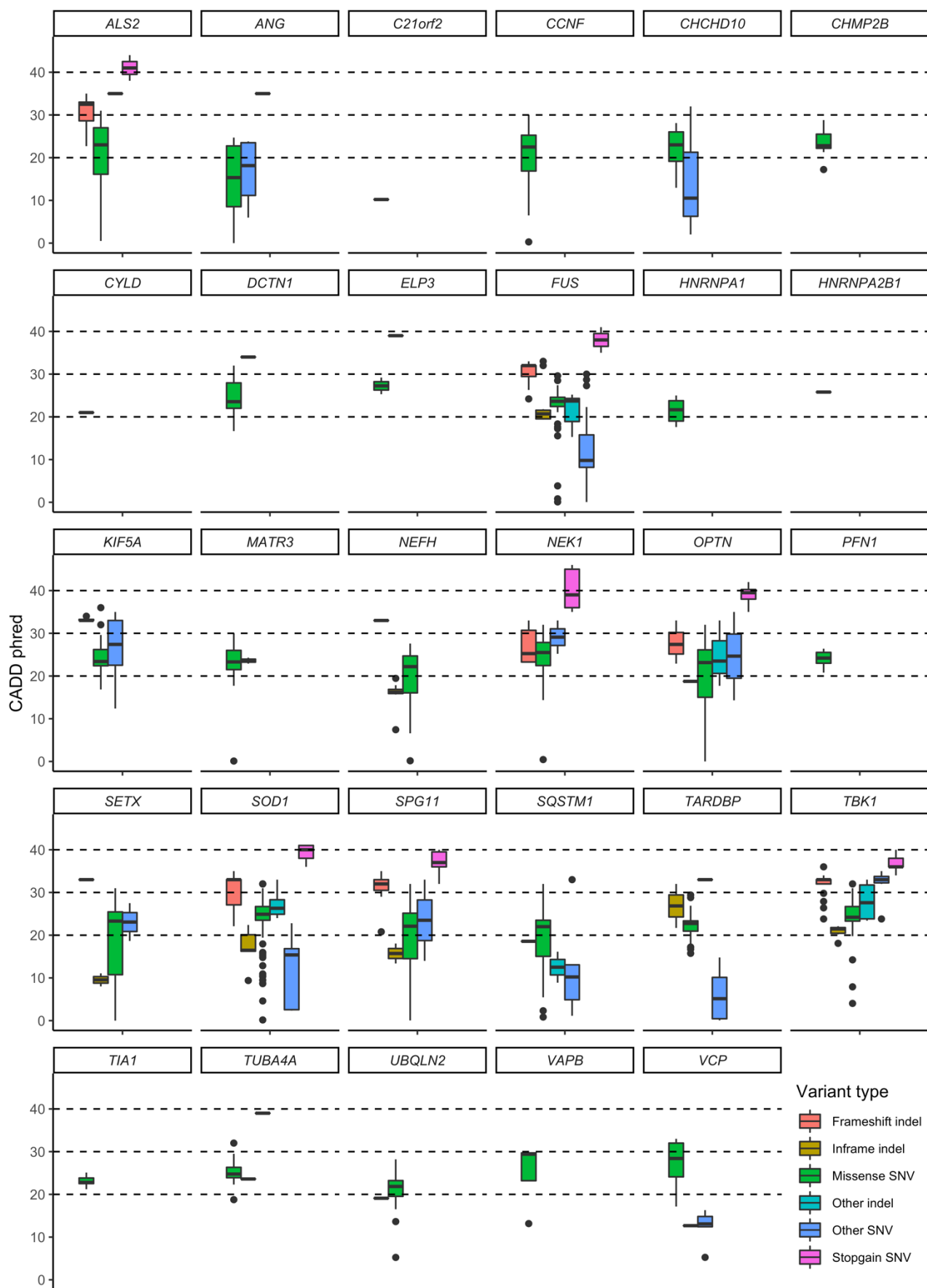
Supplementary Fig. S2. Grouped box plots of CADD phred scores for each ALS gene separated by variant type.
