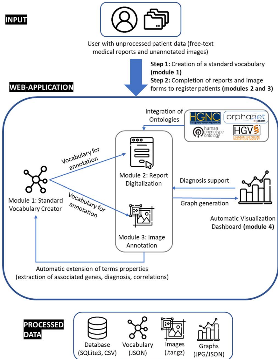
Fig. 1. Organization of IMPatient web application.
