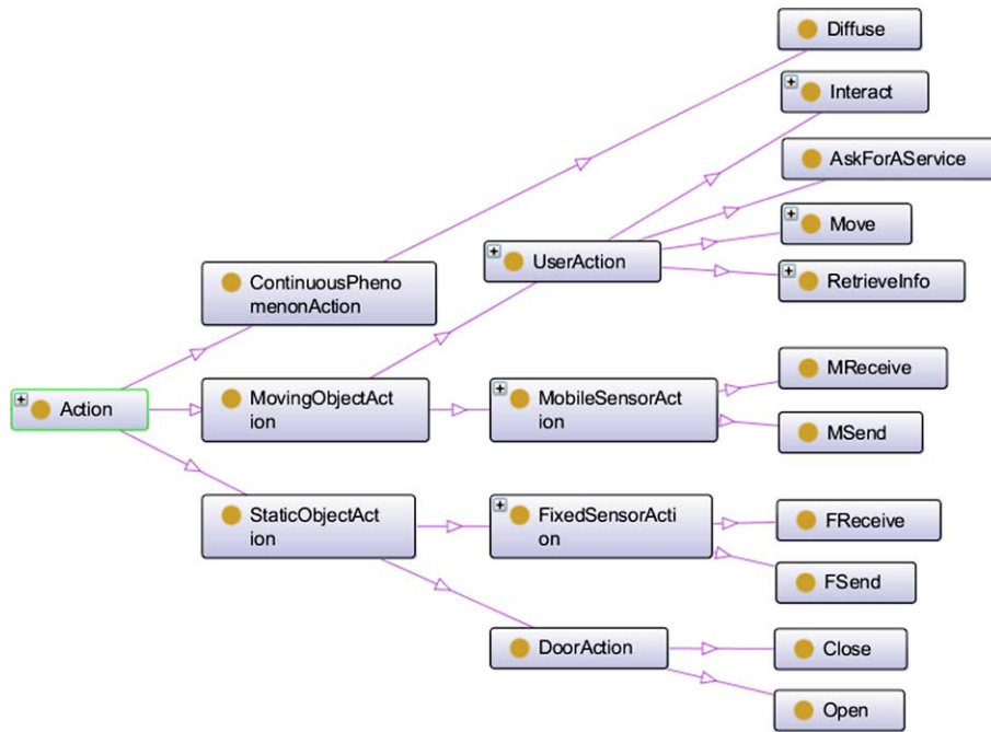
Fig. 8. A set of actions performed by different types of features.
