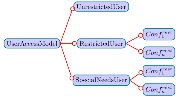
Fig. 7. Classification of user profiles based on access control information.
