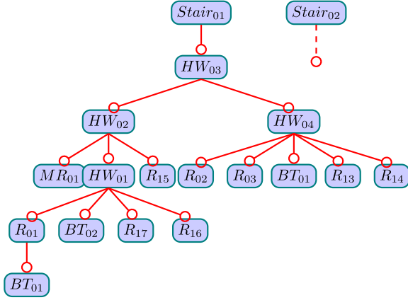
Fig. 4. Part of the location hierarchy derived from the fine-grained graph; “HW” stands for Hallway, “MR” for Meeting Room, “R” for Room, and “BT” for Bathroom.
