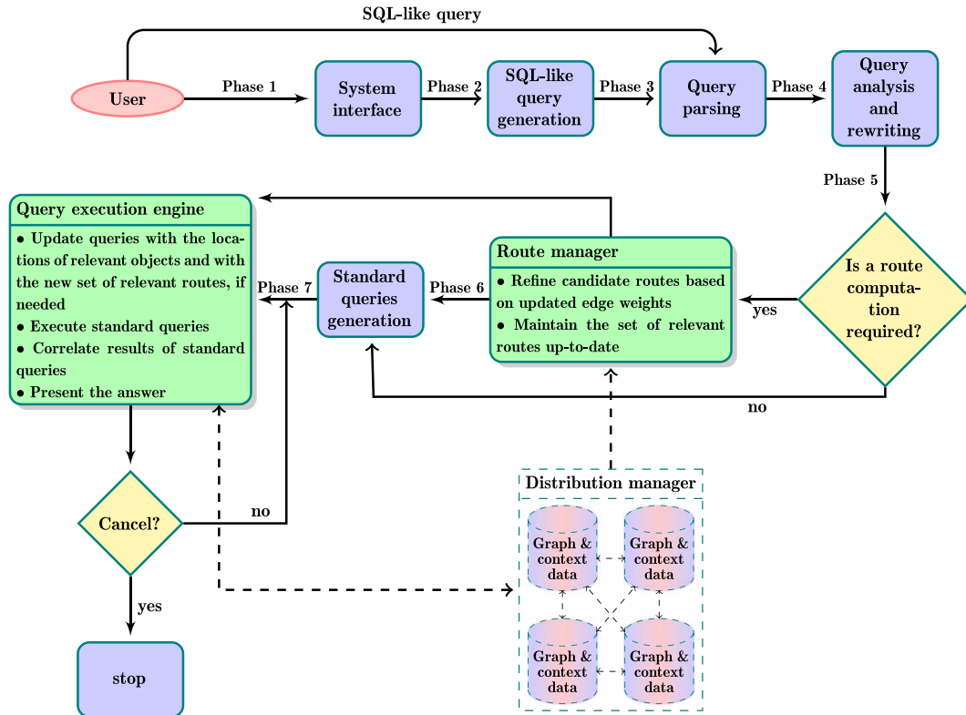
Fig. 9. Execution of location-dependent queries in indoor environments.
