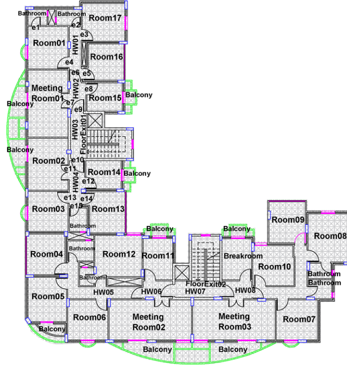
Fig. 2. A fine-grained graph of a floor plan: first level of the hierarchical spatial data model.
