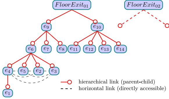
Fig. 3. Part of the exit hierarchy 4 derived from the fine-grained graph (Floor-01, Building-1).
