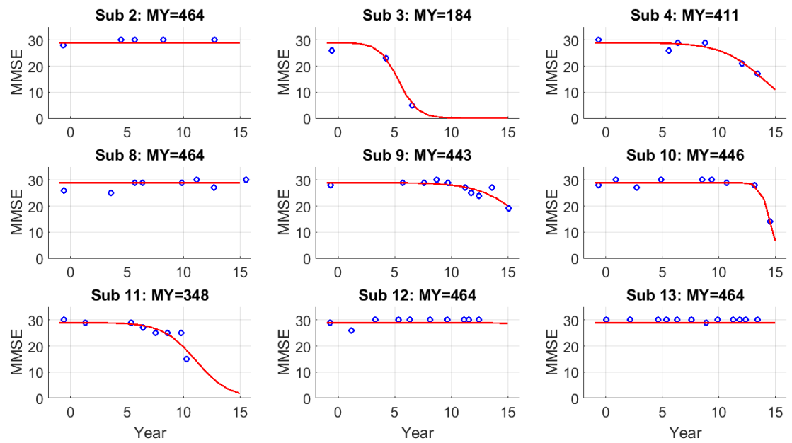
Fig. 1. MMSE Trajectories. Mini-Mental State Exam (MMSE) trajectories during follow-up period for 9 subjects from the PreC group (the ones not shown in the main paper). The x-axis labels Year with 0 corresponding to 2000. The EEG data were acquired in 1999. Blue dots denote measured MMSE scores and the red line indicates the trajectory estimated using a logistic decay model. The MY values above each plot correspond to MMSE-Years, computed as the integral under the curve.
