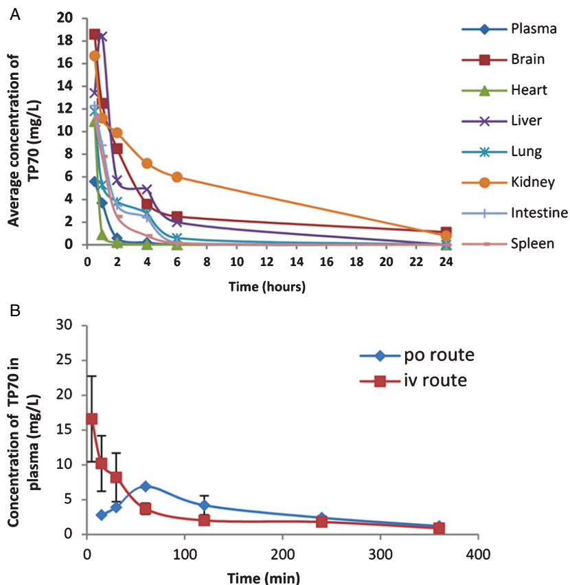
Fig. 3. Some PK properties of TP70. A) Distribution of TP70 in various tissues and plasma after i.p. administration in 3-month-old male WT C57BL/6 mice (25 mg/Kg body weight) from 0–24 h. Shown are the means from three mice per time point. B) The concentrations of TP70 in plasma following i.v. and p.o. administration.
