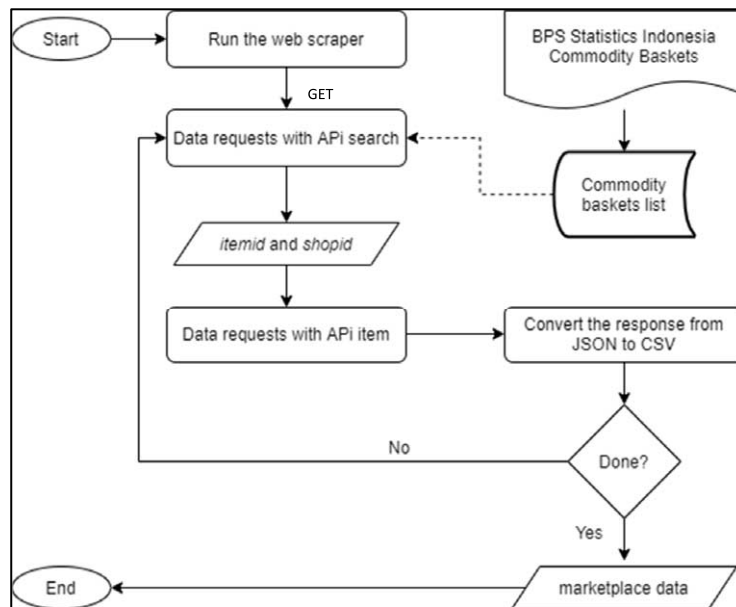
Fig. 4. Data extraction flow.
