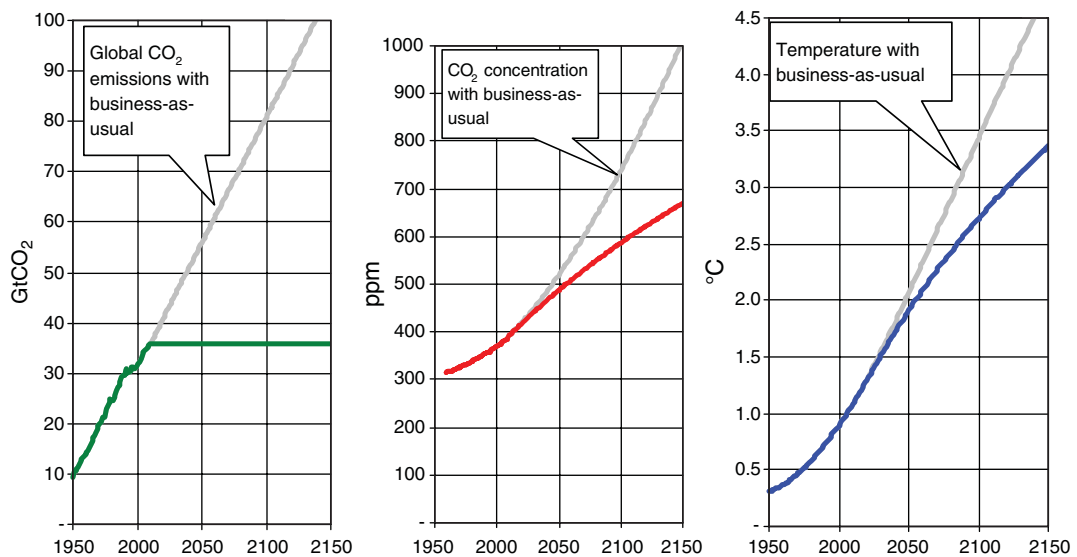
Fig. 1. The diagram on the left shows a linearly increasing global emissions business-as-usual scenario (grey curve) and a scenario that stabilizes global emissions at current levels (colored curve). Under the latter scenario, the CO 2 concentration in the atmosphere would continue to grow (middle diagram). So would the global temperature (diagram on right). (Source: see footnote 5 in article.)
