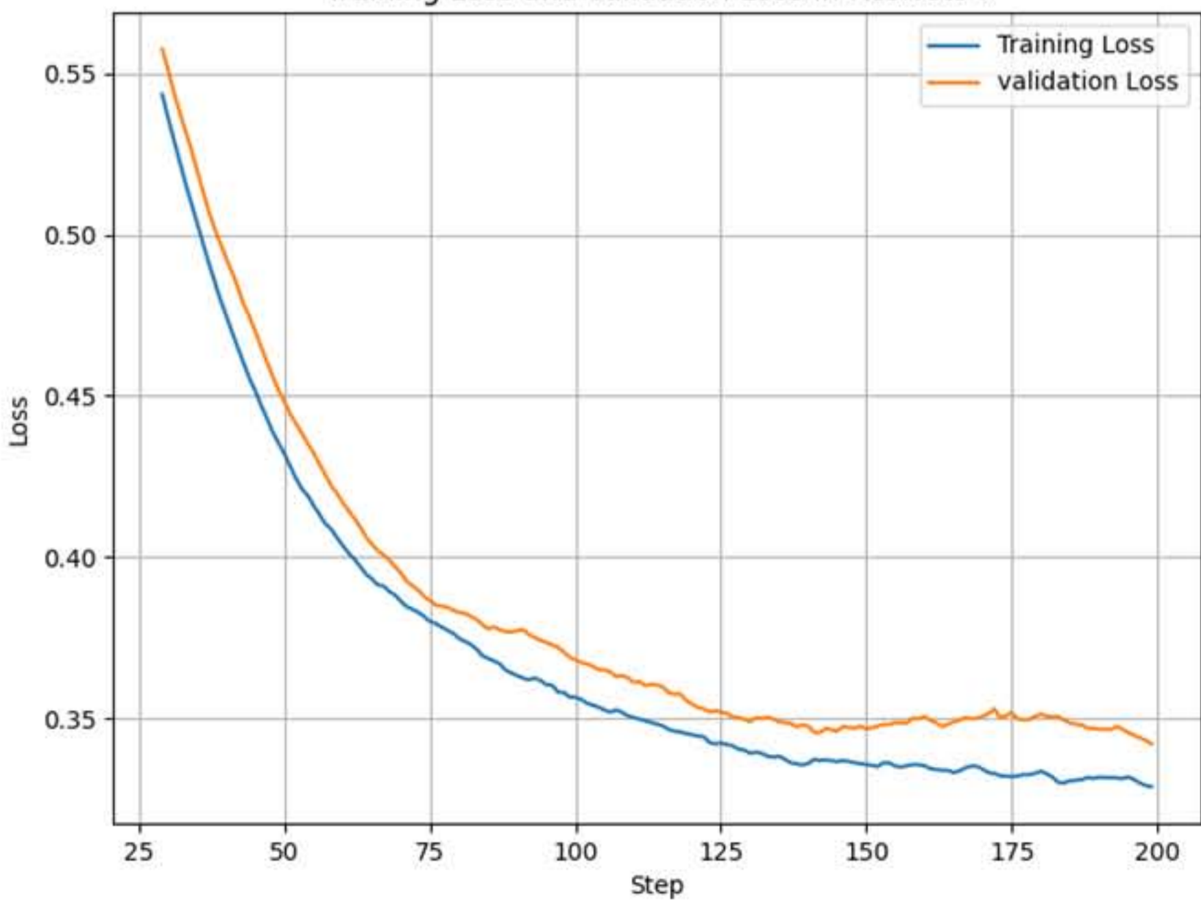
Training Loss and Validation Loss in ResNet34
