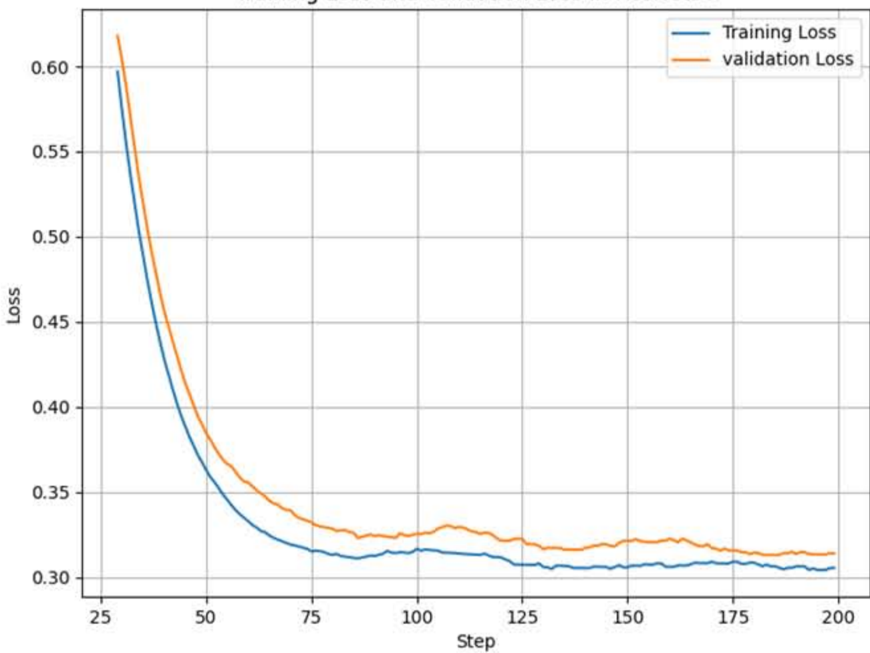
Training Loss and Validation Loss in ResNet50
