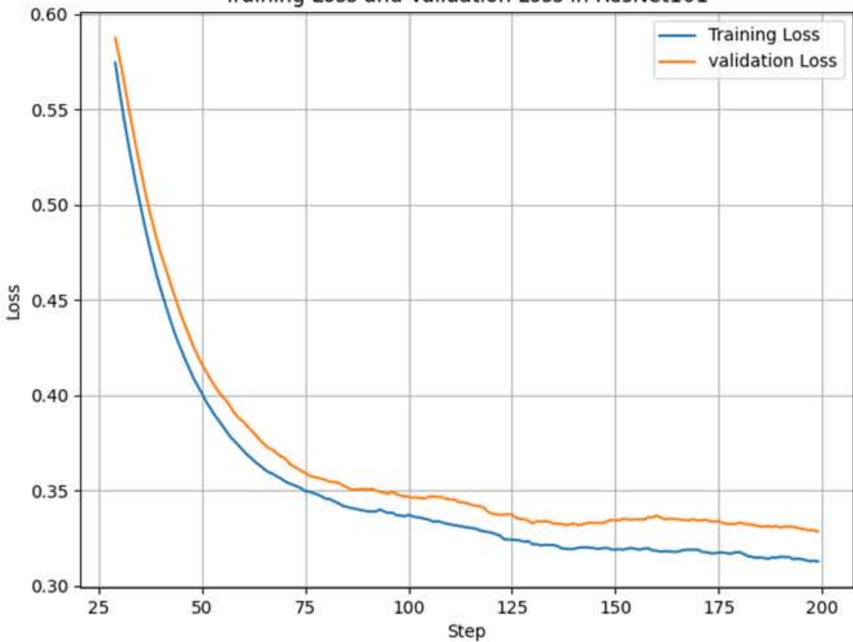
Training Loss and Validation Loss in ResNet101
